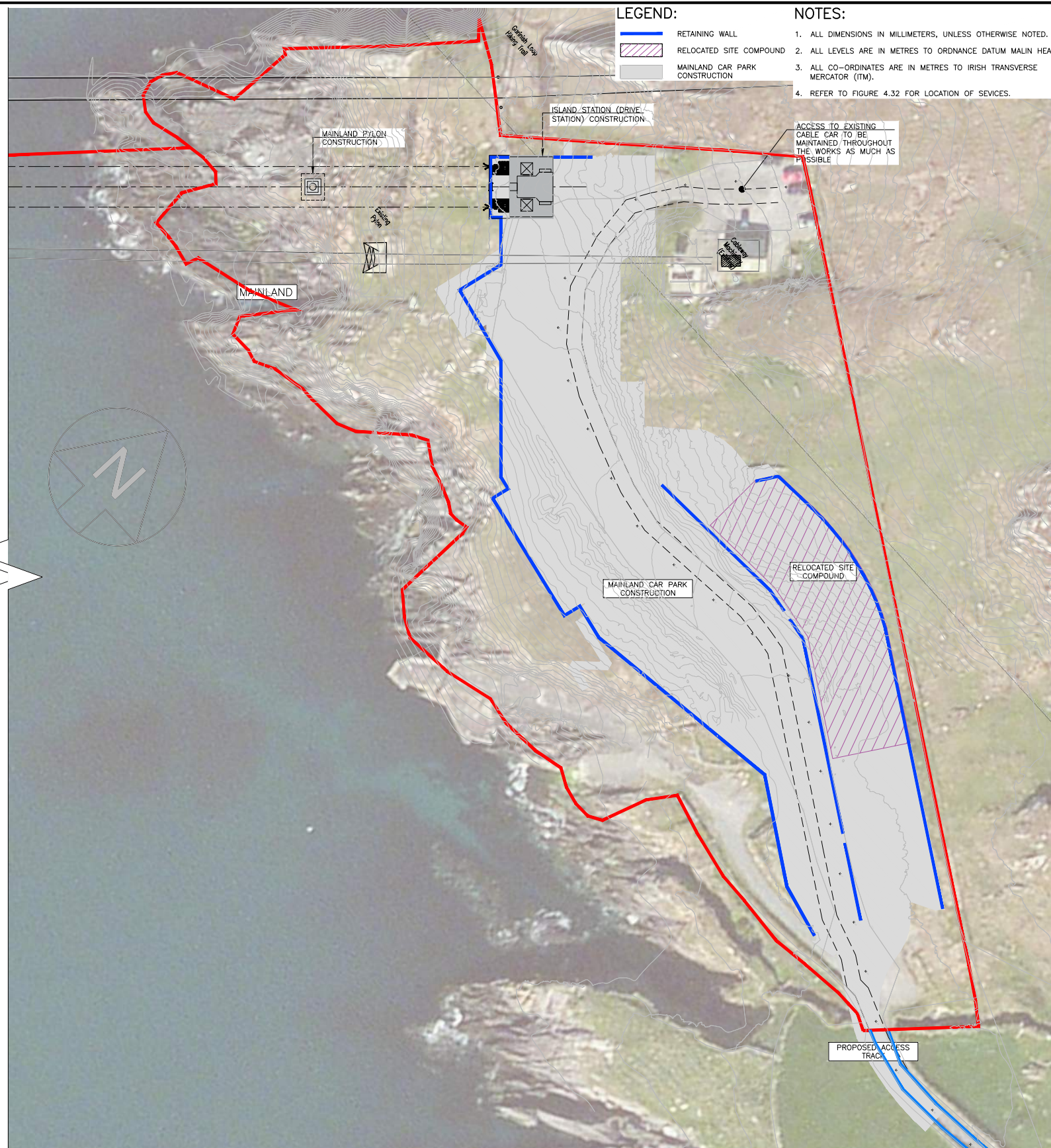
CONSTRUCTION OF CABLEWAY STAGE 3 A1 SCALE - 1:500 A3 SCALE - 1:1000
